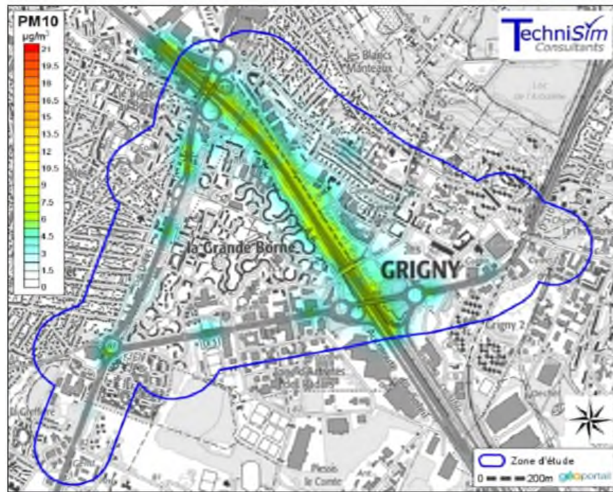
Figure 173 – Horizon 2025 projet– concentration ( \mu\text{g}/\text{m}^3 ) moyenne annuelle PM10
